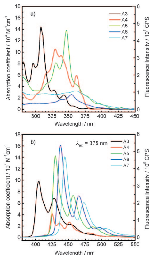
Figure 3. a) UV/Vis absorption spectra of A3–A7 in CH 2 Cl 2 . b) Unnormalized fluorescence spectra obtained at excitation of 375 nm.
