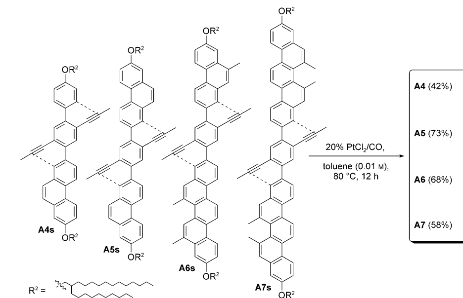
Scheme 3. Platinum-catalyzed regiocontrolled synthesis of series A .
